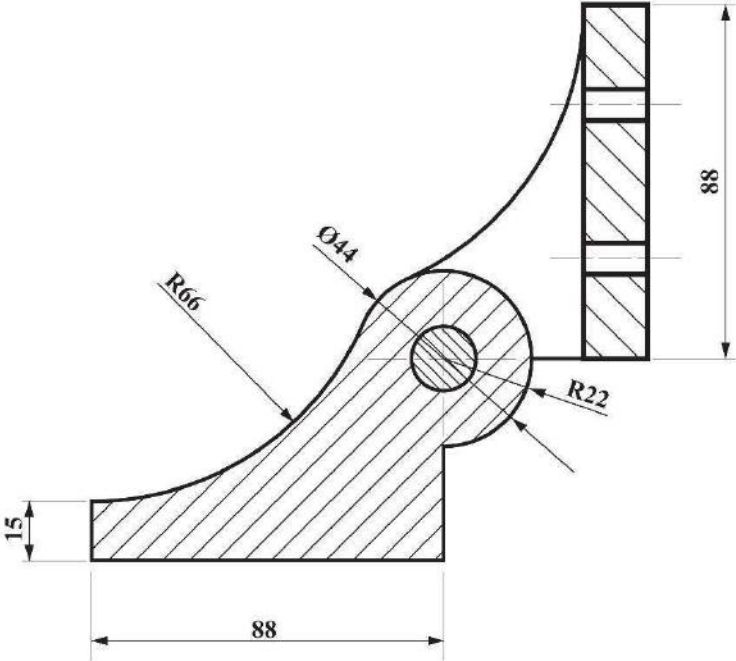
SECTIONAL ELEVATION A - A
